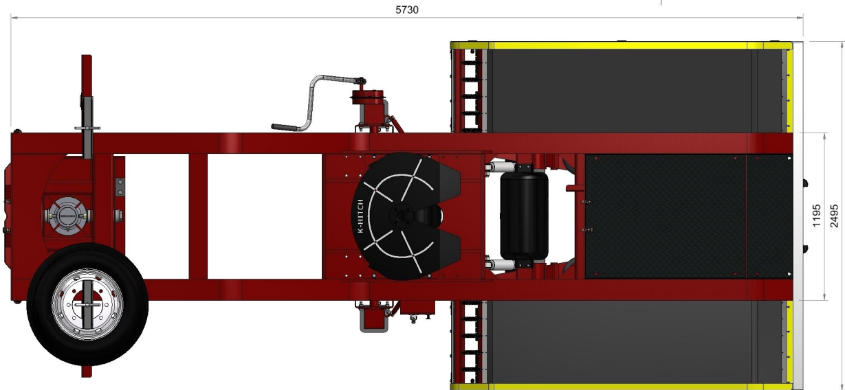
TOP VIEW TANDEM AXLE LOW LOADER DOLLY
