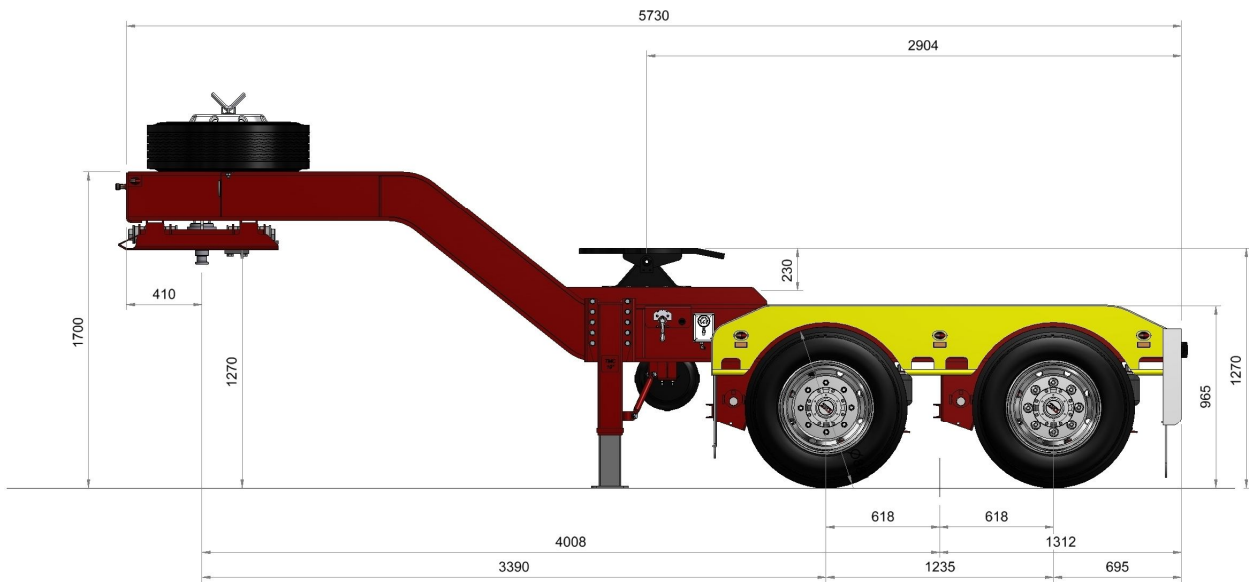
PASSENGER'S SIDE VIEW TANDEM AXLE LOW LOADER DOLLY
