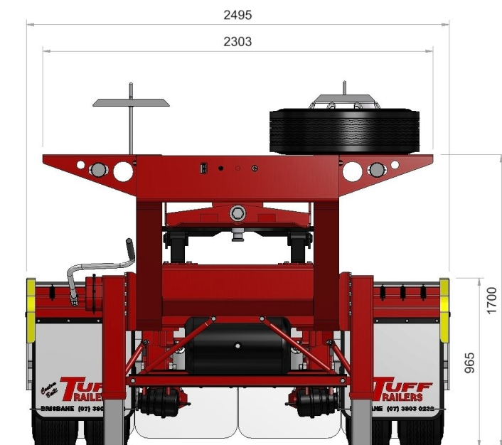
FRONT VIEW TANDEM AXLE LOW LOADER DOLLY
